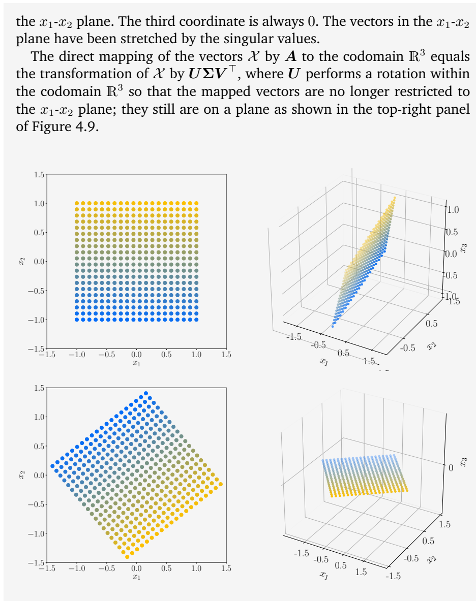
Figure 4.9 SVD and mapping of vectors (represented by discs). The panels follow the same anti-clockwise structure of Figure 4.8.
