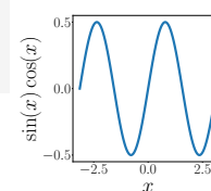
Figure 3.8 f(x) = \sin(x) \cos(x) .
